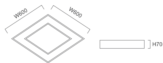
KA-5215 LED
